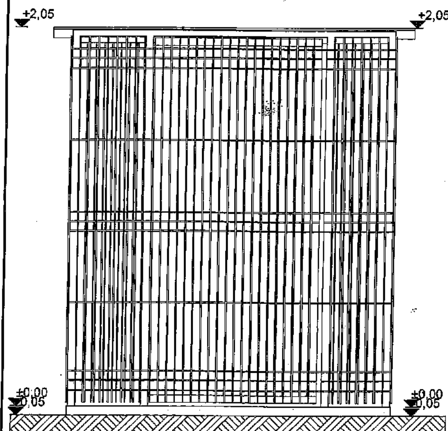
FATADA PRINCIPALA scara 1:20
